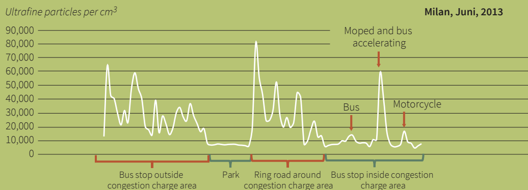
Figure 7: Measurements of ultrafine particles to assess the congestion charge area in Milan.
