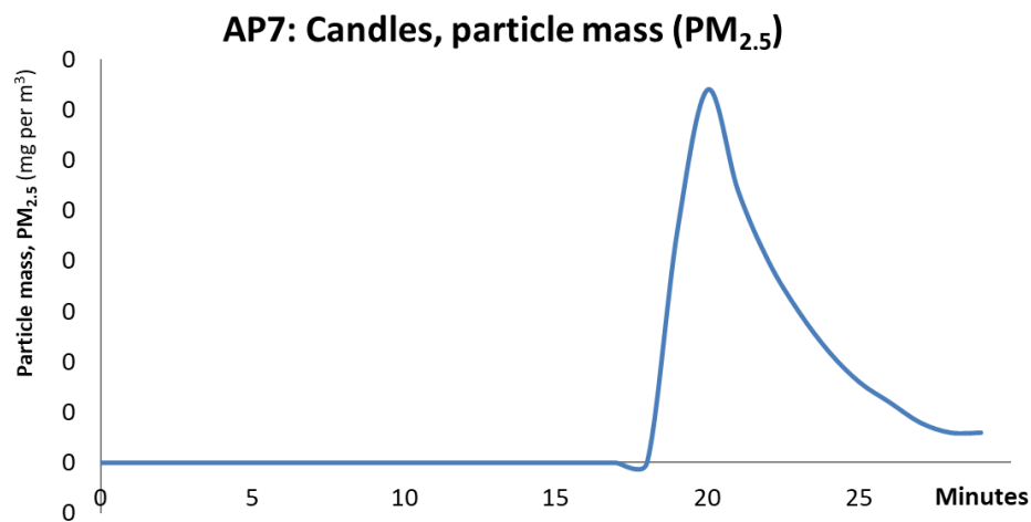
Figure 2.7.5: Particle mass (PM 2.5 ) – DustTrak on bed
