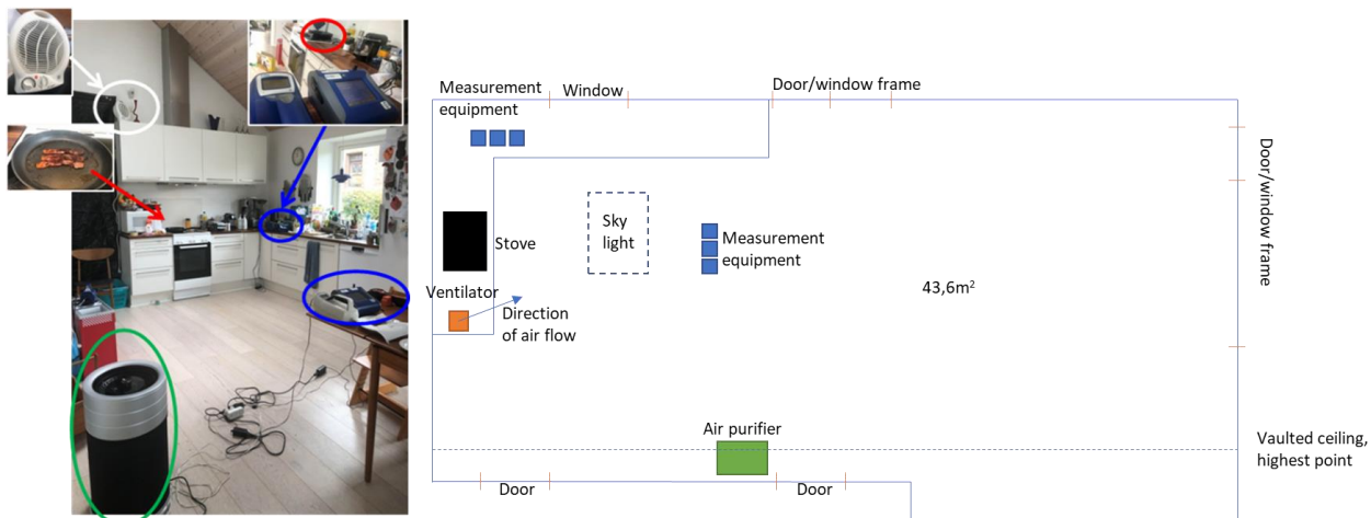
Figure 1: Photos and sketch of set-up in the living room-kitchen-dining area.
