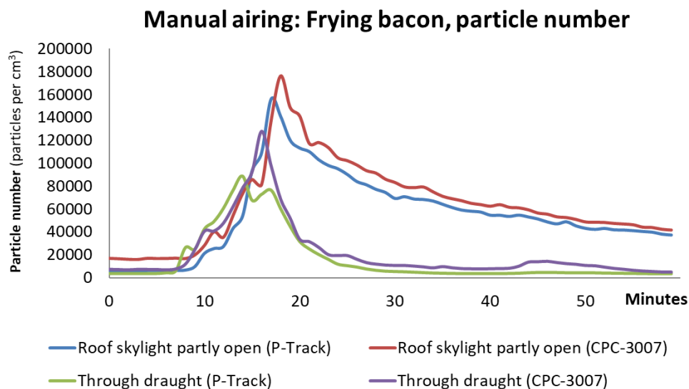
Figure 2.10.1: Particle number (P-Track on kitchen table and CPC-3007 on dining table).
