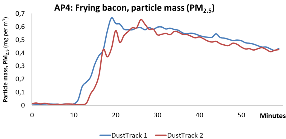
Figure 2.4.2: Particle mass, PM 2.5 (Dust Trak 1 on kitchen table and Dust Trak 2 on dining table).
