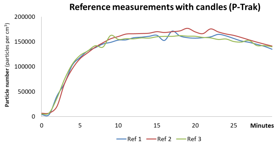
Figure 1.6: Particle number - P-Trak on bed
