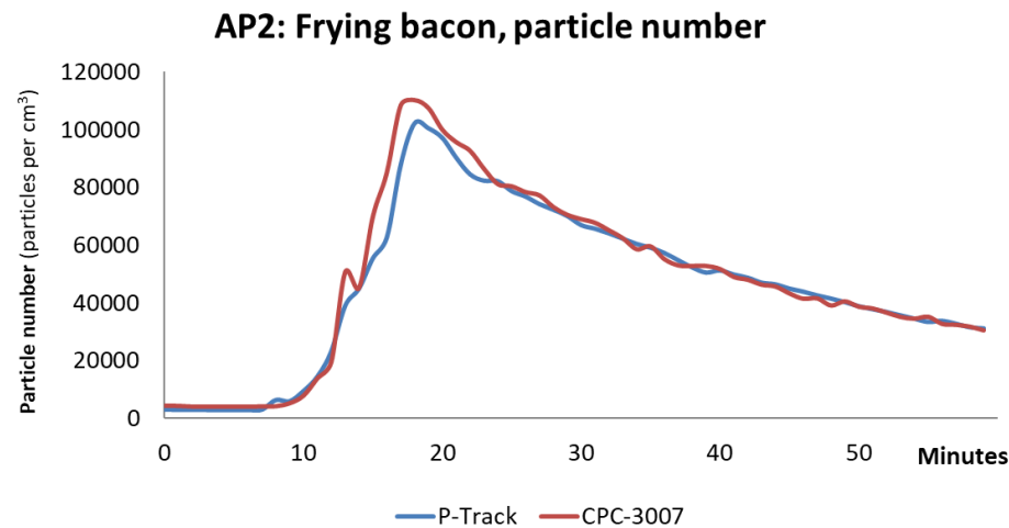
Figure 2.2.1: Particle number (P-Track on kitchen table and CPC-3007 on dining table).
