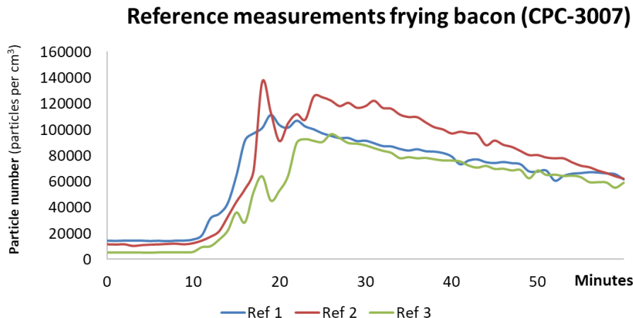
Figure 1.2: Particle number - CPC-3007 on dining table
