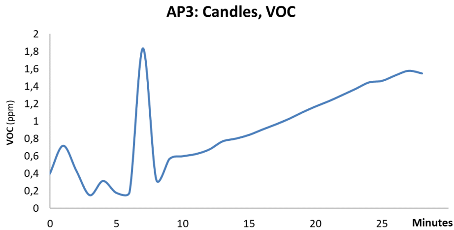
Figure 2.3.6: VOCs – Tiger TVOC Detector on bed
