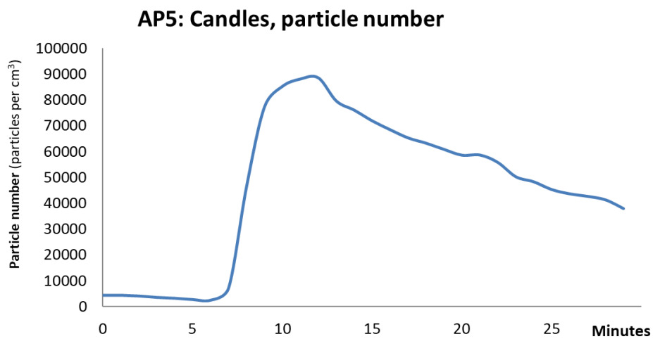
Figure 2.5.4: Particle number (P-Track on bed).
