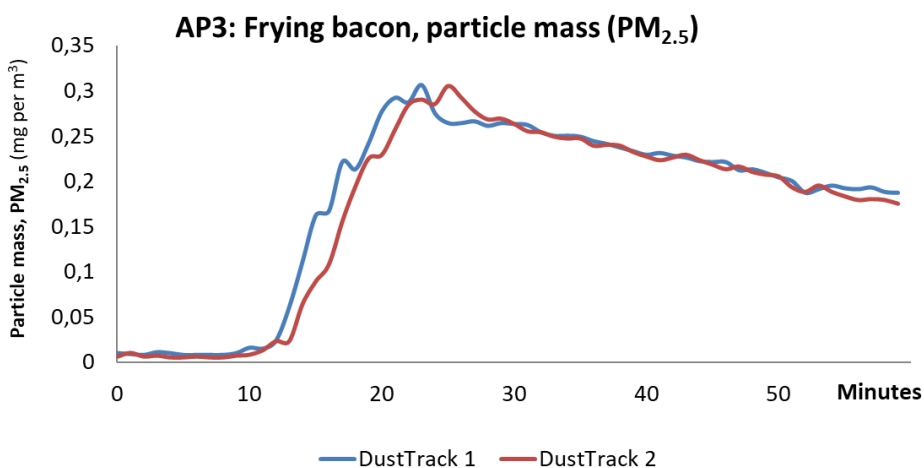
Figure 2.3.2: Particle mass, PM 2.5 (Dust Trak 1 on kitchen table and Dust Trak 2 on dining table).
