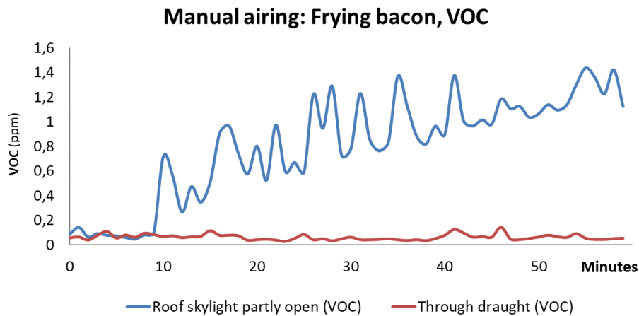
Figure 2.10.3: VOCs (Tiger TVOC Detector on dining table).
