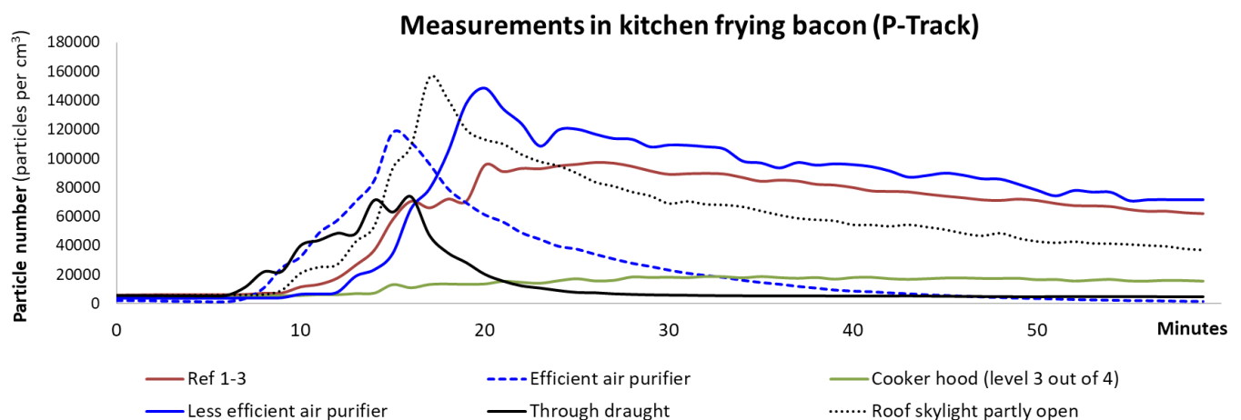
Figure 3: Particle number in kitchen measurements
