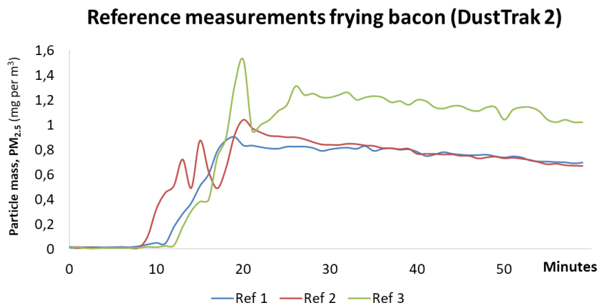
Figure 1.4: Particle mass (PM 2.5 ) - DustTrak on dining table
