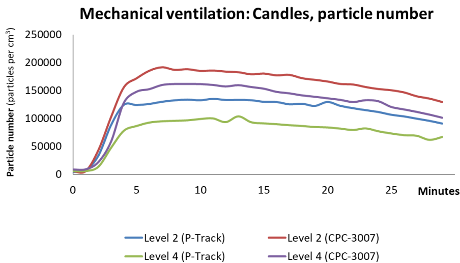
Figure 2.11.1: Particle number (P-Track and CPC-3007 on bed).
