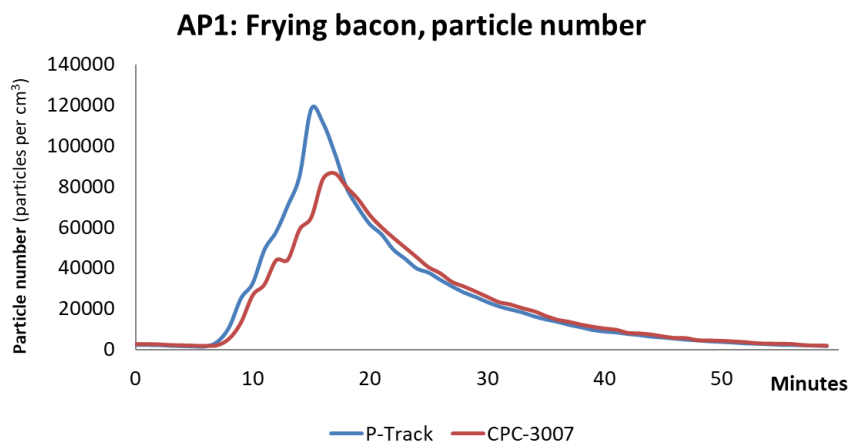
Figure 2.1.1: Particle number (P-Track on kitchen table and CPC-3007 on dining table).
