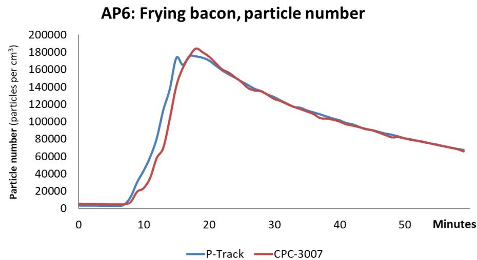
Figure 2.6.1: Particle number (P-Track on kitchen table and CPC-3007 on dining table).
