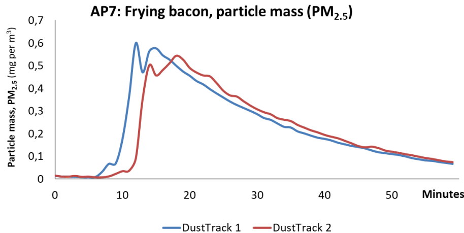
Figure 2.7.2: Particle mass, PM 2.5 (Dust Trak 1 on kitchen table and Dust Trak 2 on dining table).
