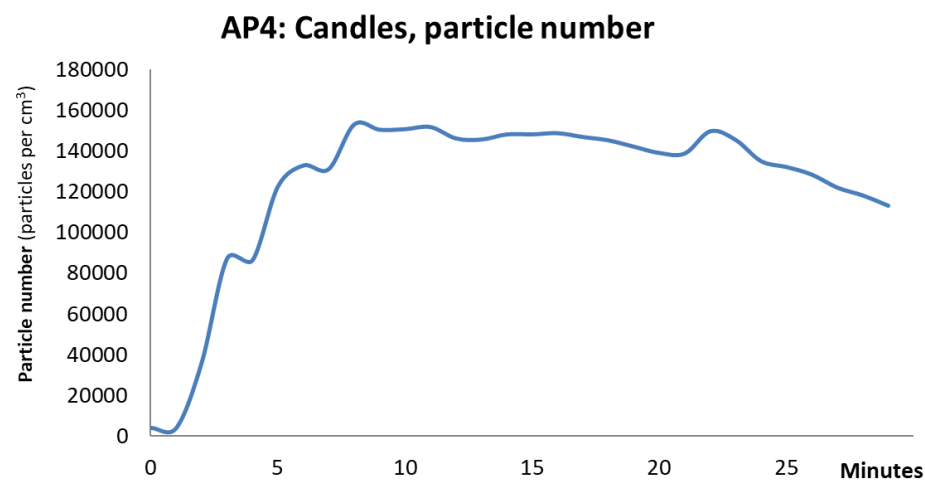
Figure 2.4.4: Particle number (P-Track on bed).
