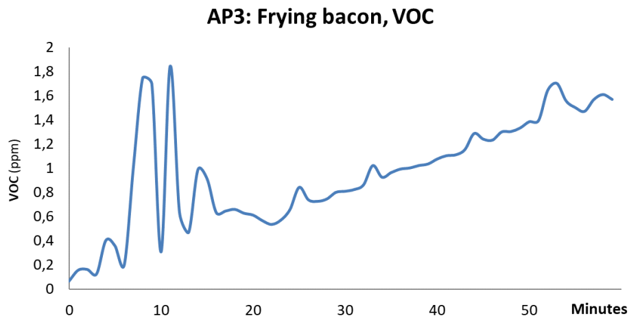
Figure 2.3.3: VOCs (Tiger TVOC Detector on dining table).
