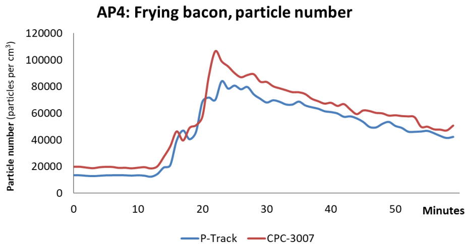
Figure 2.4.1: Particle number (P-Track on kitchen table and CPC-3007 on dining table).
