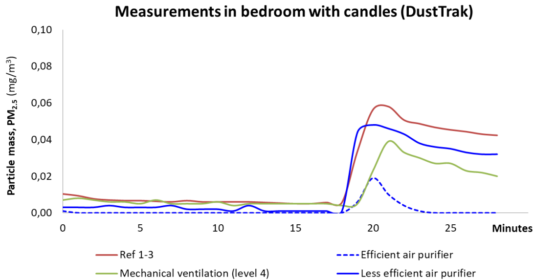
Figure 6: Particle mass (PM 2.5 ) in bedroom measurements
