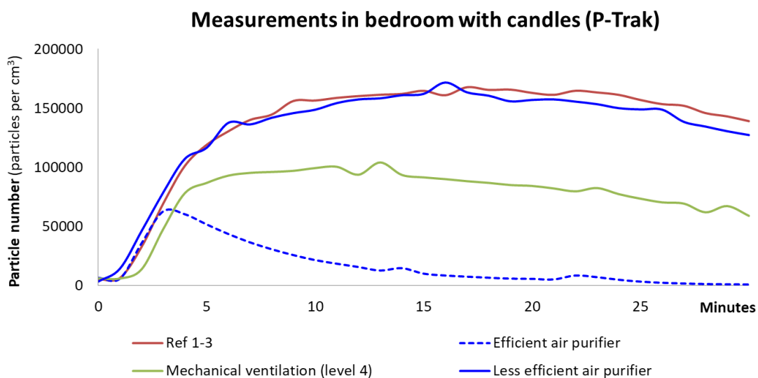
Figure 5: Particle number in bedroom measurements
