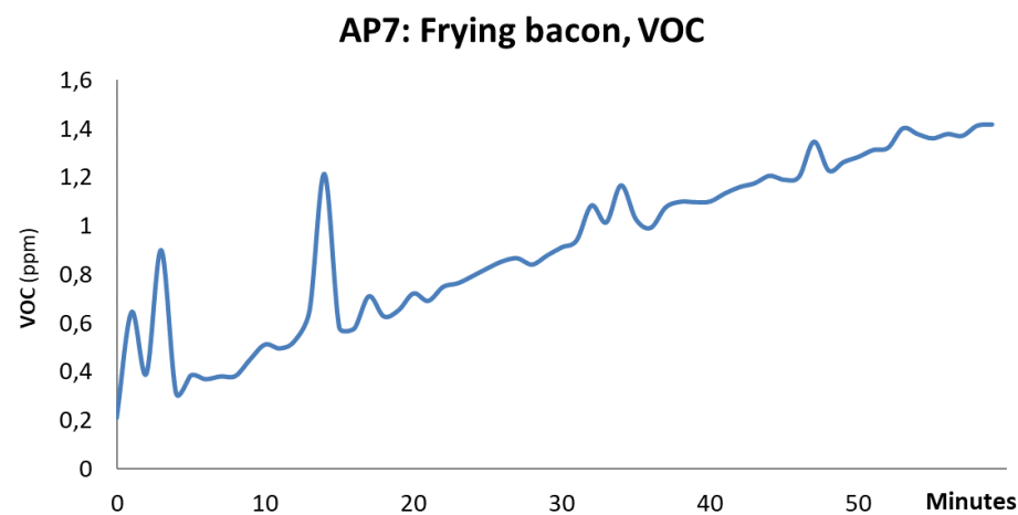
Figure 2.7.3: VOCs (Tiger TVOC Detector on dining table).
