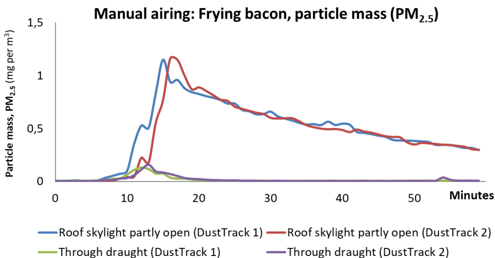
Figure 2.10.2: Particle mass, PM_{2.5} (Dust Trak 1 on kitchen table and Dust Trak 2 on dining table).
