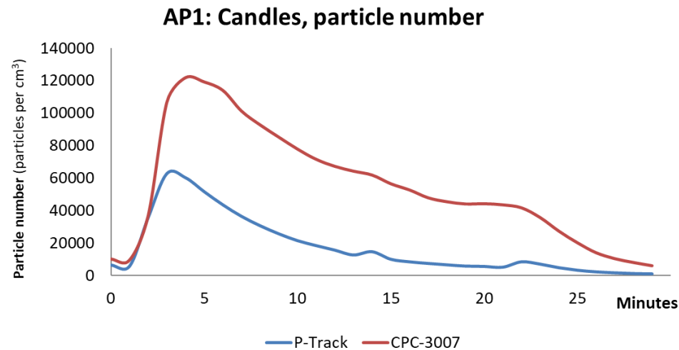
Figure 2.1.4: Particle number (P-Track and CPC-3007 on bed).
