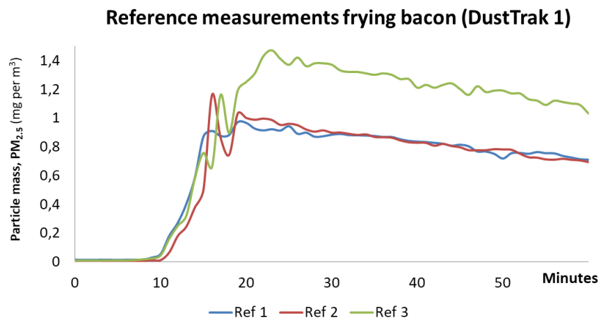
Figure 1.3: Particle mass (PM 2.5 ) - DustTrak on kitchen table
