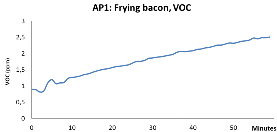
Figure 2.1.3: VOCs (Tiger TVOC Detector on dining table).
