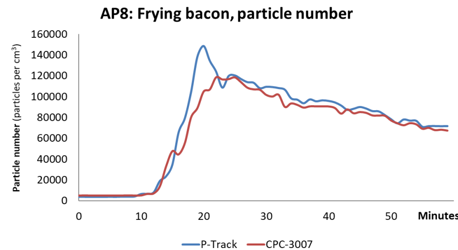
Figure 2.8.1: Particle number (P-Track on kitchen table and CPC-3007 on dining table).
