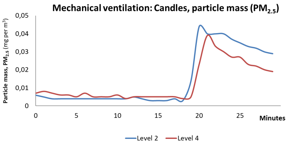
Figure 2.11.2: Particle mass ( PM_{2.5} ) - DustTrak on bed
