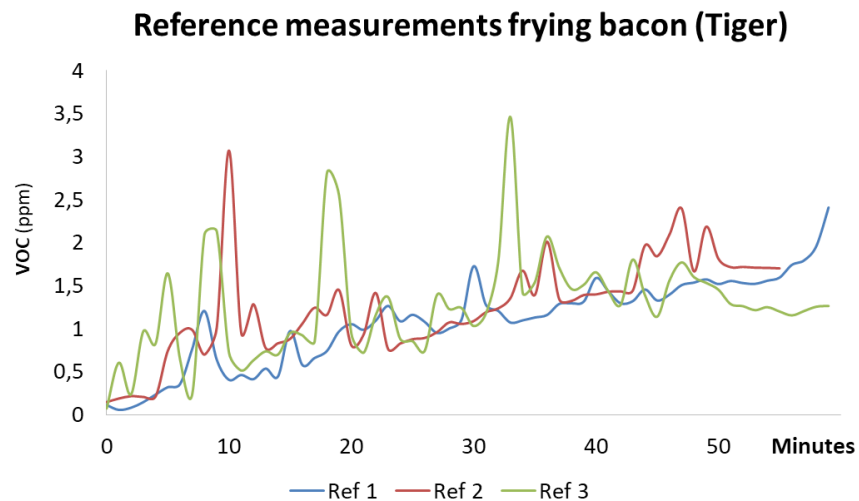
Figure 1.5: VOCs – Tiger TVOC Detector on dining table
