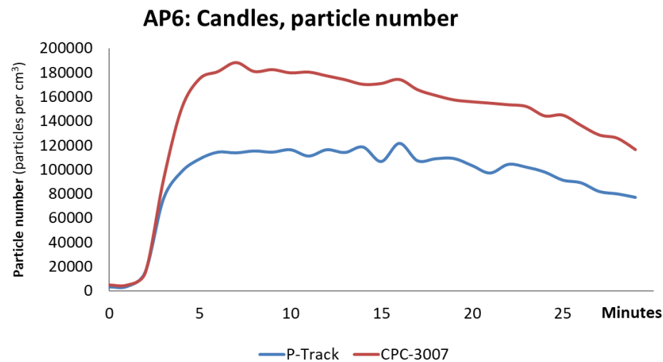
Figure 2.6.4: Particle number (P-Track and CPC-3007 on bed).
