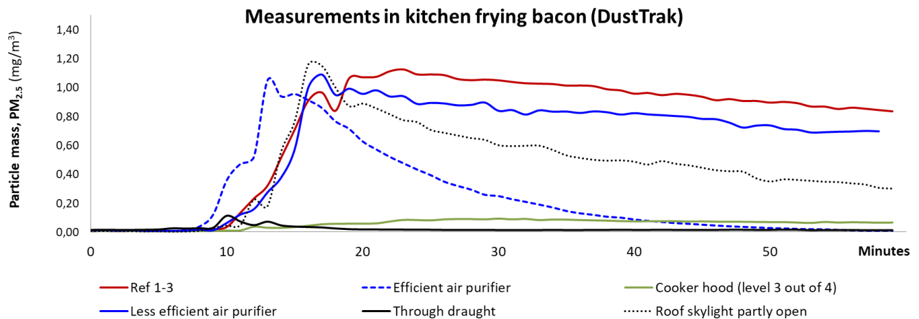
Figure 4: Particle mass (PM 2.5 ) in kitchen measurements
