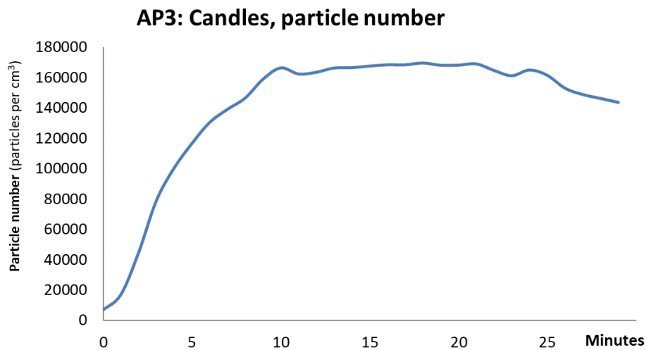
Figure 2.3.4: Particle number (P-Track on bed).
