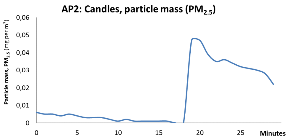
Figure 2.2.5: Particle mass (PM 2.5 ) - DustTrak on bed
